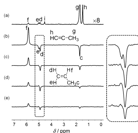
Figure 4. 400 MHz 1 H NMR spectra (90° RF pulse flip angle) of products resulting from PY hydrogenation over shaped ceria nanocrystals. a) Thermally polarized spectrum of the products of hydrogenation over ceria nanocubes with n-H 2 at 300 °C. Note the eightfold amplification of the vertical scale relative to the other spectra in this Figure. Peak i was assigned to an alkadiene, as reported previously. [29] b) ALTADENA spectrum (32 scans) resulting from hydrogenation over nanocubes at 300 °C using p-H 2 . c–e) ALTADENA spectra acquired for the hydrogenation over nanocubes (c), nano-octahedra (d), or nanorods (e) at 375 °C with p-H 2 . Inset: Expansion of the PE CH 2 (H d and H e ) region exhibiting syn addition stereoselectivity.
